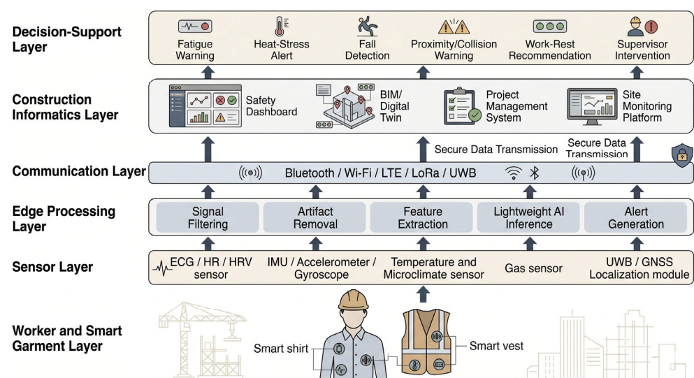
Figure 1. Layered cyber–physical architecture of sensor-integrated smart garments for construction safety.
